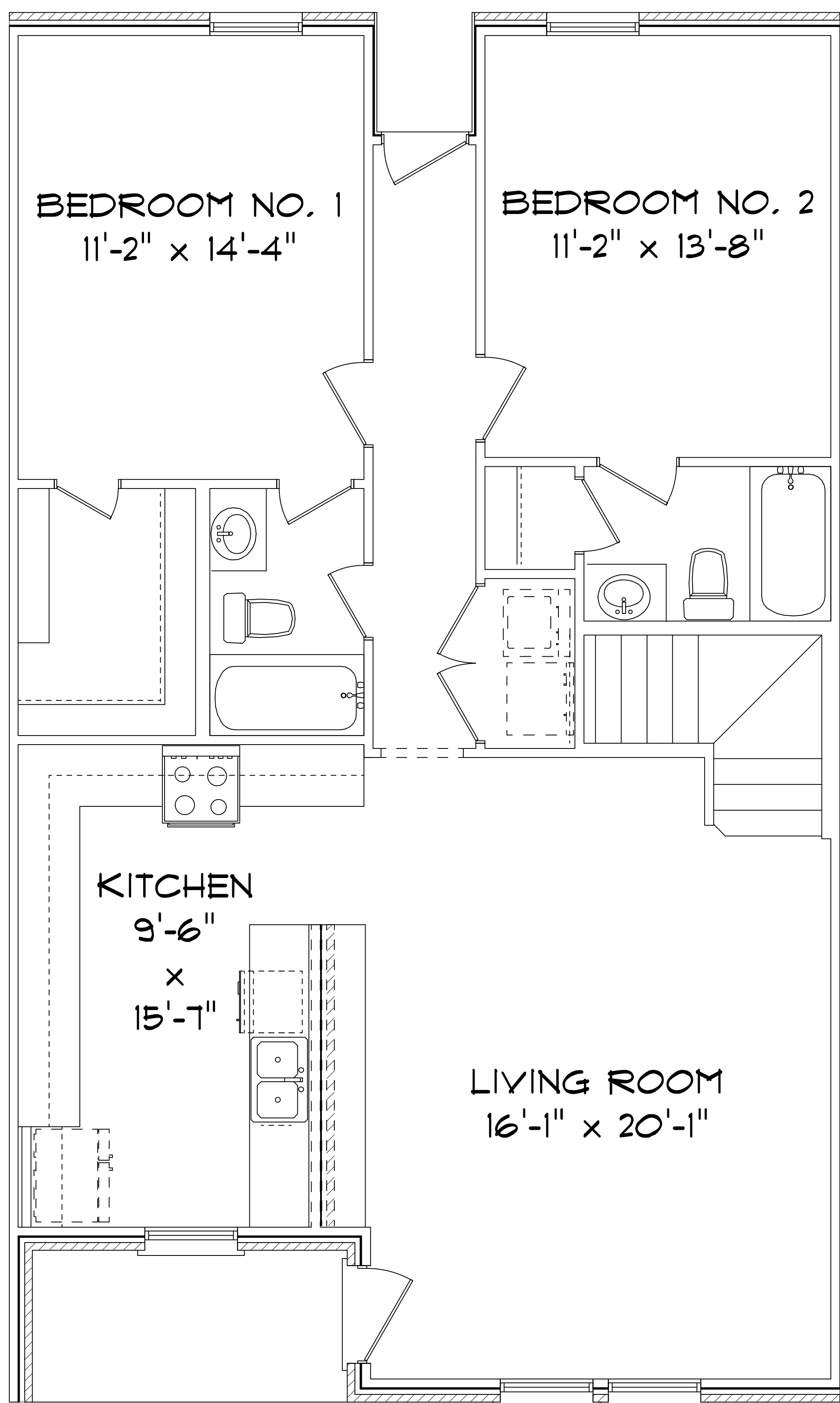
First Floor
